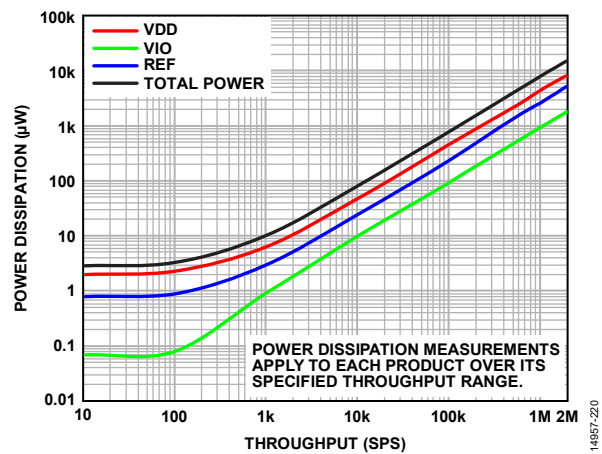
Figure 35. Power Dissipation vs. Throughput, VIO = 1.8 V
