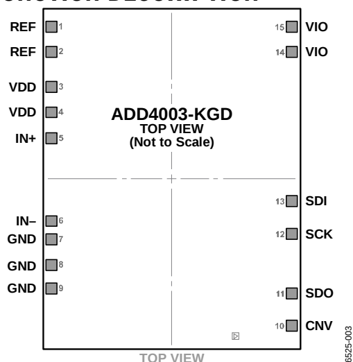
Figure 3. Pad Configuration
