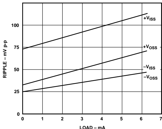
Figure 16a. Isolated Supply Ripple vs. Load (External 4.7\text{ }\mu\text{F} Bypass)
