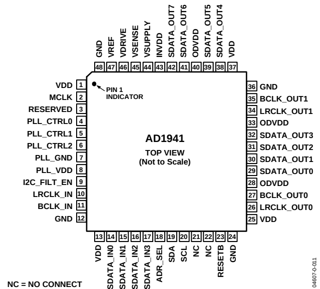
Figure 8. 48-Lead LQFP Pin Configuration, AD1941
