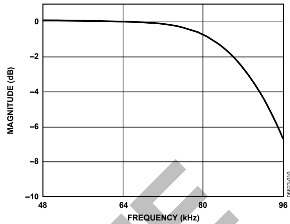
Figure 10. DAC Stop-Band Filter Response, 192 kHz
