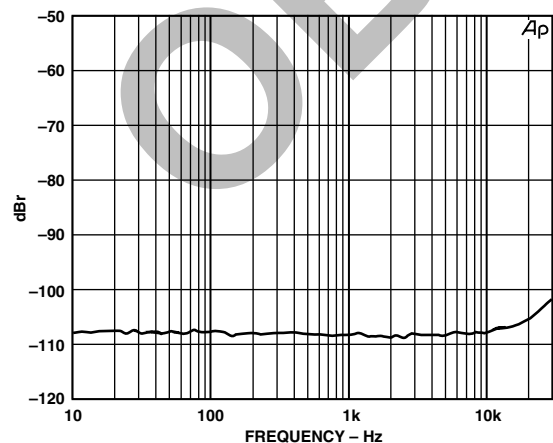
Figure 13. THD vs. Frequency Input @ -3 dBFS, SR 48 kHz
