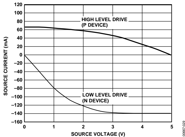
Figure 29. ADSP-2106x Typical Drive Currents ( V_{DD} = 5V )
