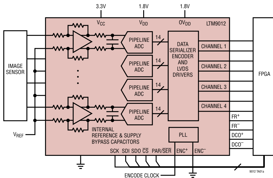
Single-Ended Sensor Digitization
