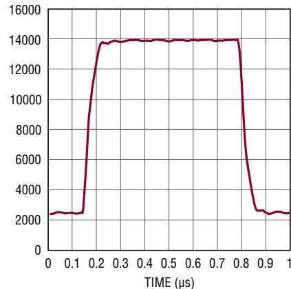
Pulse Response
