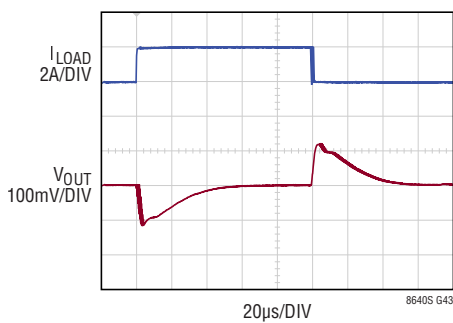
LT8640S Transient Response; Internal Compensation
