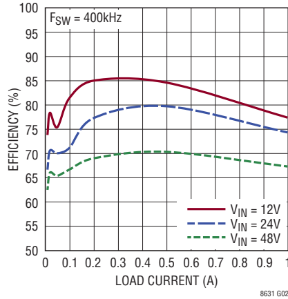
Efficiency at V_{OUT} = 3.3V
