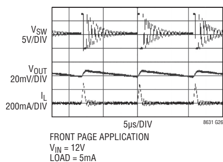
Burst Waveforms
