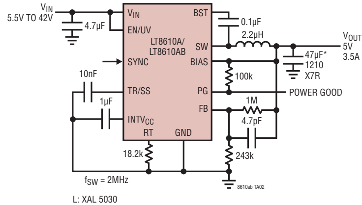
5V 2MHz Step-Down Converter
