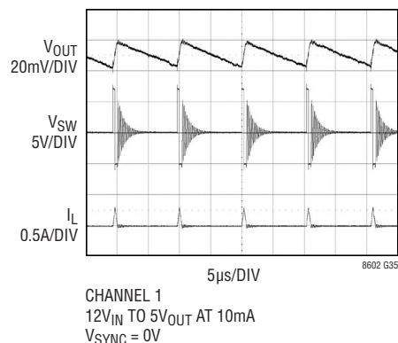
Light Load Waveforms
