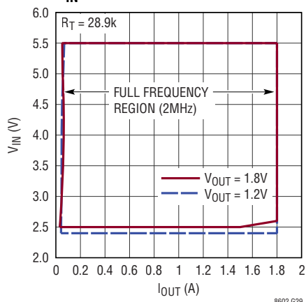
Channel 3, 4 Full Frequency V_{IN} vs Load Current
