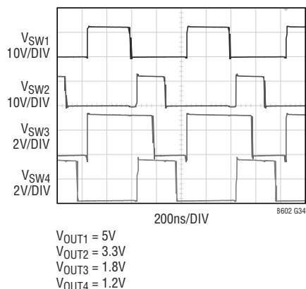
Full Frequency Waveforms
