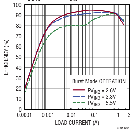
LV Channel Efficiency vs Load V_{OUT3} = 1.8V , f_{SW} = 1MHz
