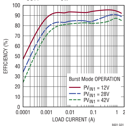
Channel 1 Efficiency vs Load V_{OUT1} = 8V , f_{SW} = 2MHz
