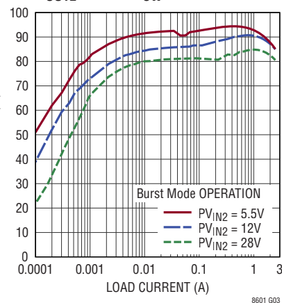
Channel 2 Efficiency vs Load V_{OUT2} = 3.3V , f_{SW} = 1MHz
