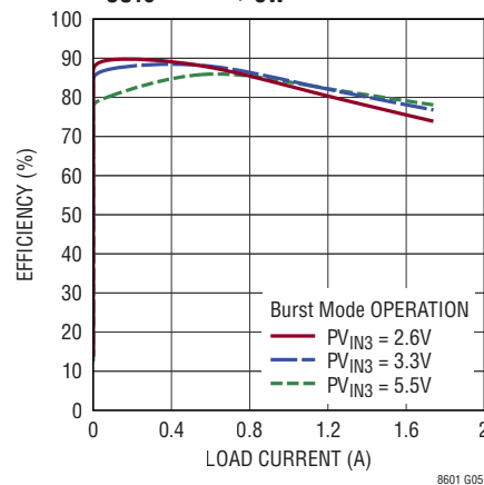
LV Channel Efficiency vs Load V_{OUT3} = 1.2V , f_{SW} = 2MHz
