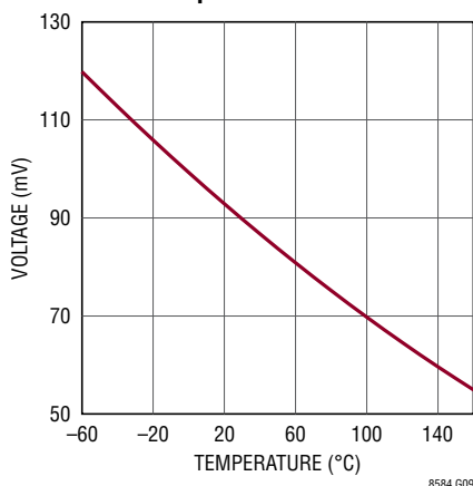
DCM Comparator Threshold
