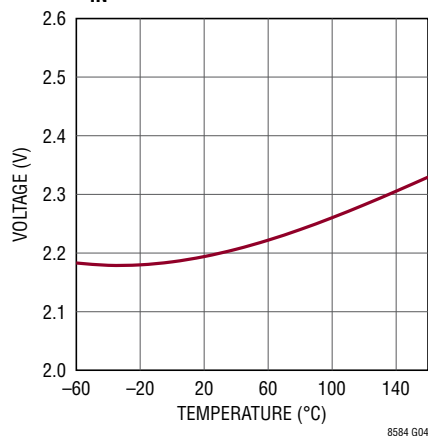
V_{IN} Internal UVLO
