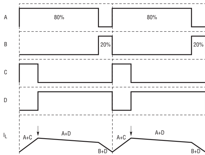
Figure 6. Peak-Boost in Buck-Boost Region ( V_{IN} < V_{OUT} )
