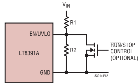
Figure 12. V_{IN} Undervoltage Lockout (UVLO)
