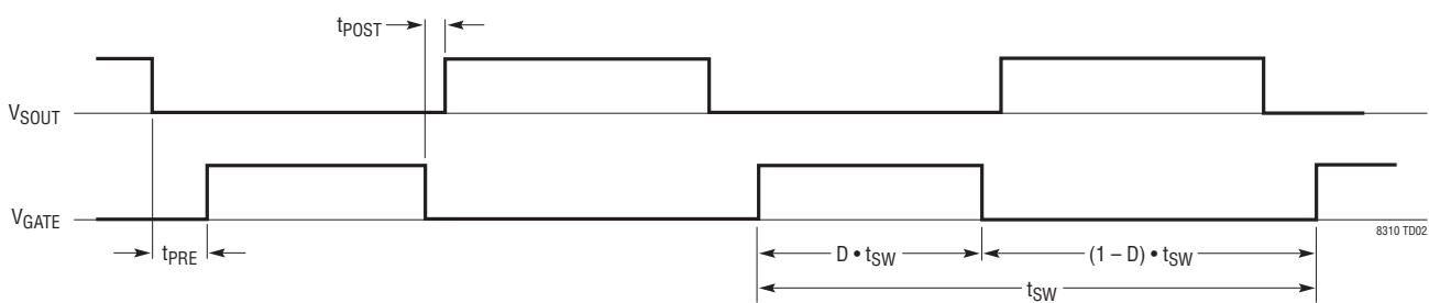
Nonoverlapping GATE/SOUT
