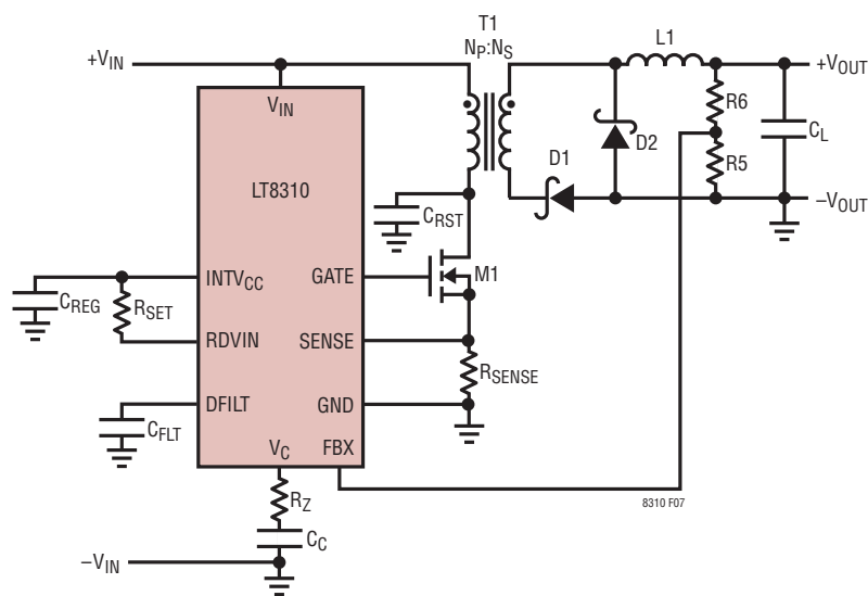
Figure 7. Forward Nonsynchronous Direct-Wired Nonisolated Basic Schematic
