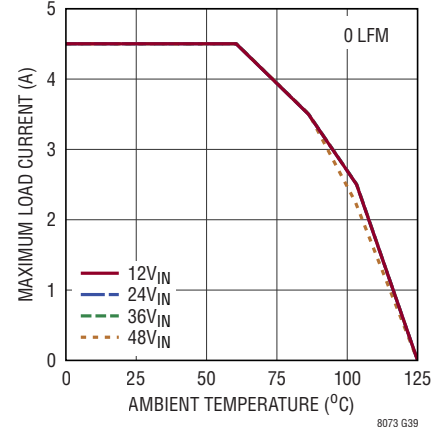
Derating, V_{OUT} = 0.8V , BIAS = 5V, DC2389A Demo Board
