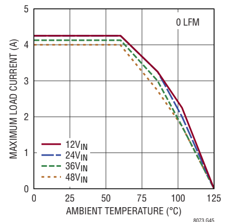
Derating, V_{OUT} = 3.3V , BIAS = 5V, DC2389A Demo Board
