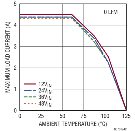
Derating, V_{OUT} = 1.5V , BIAS = 5V, DC2389A Demo Board
