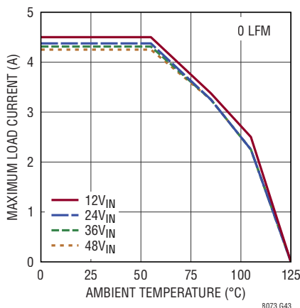
Derating, V_{OUT} = 1.8V , BIAS = 5V, DC2389A Demo Board
