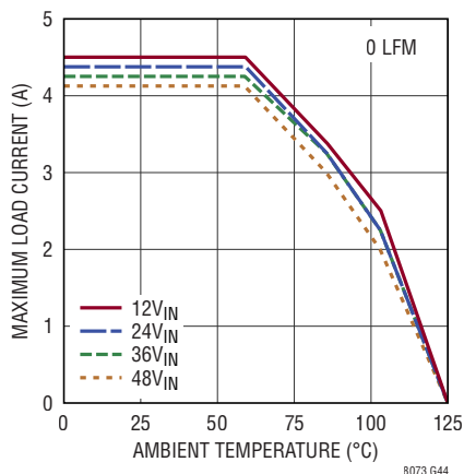
Derating, V_{OUT} = 2.5V , BIAS = 5V, DC2389A Demo Board
