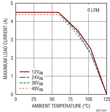
Derating, V_{OUT} = 1.2V , BIAS = 5V, DC2389A Demo Board
