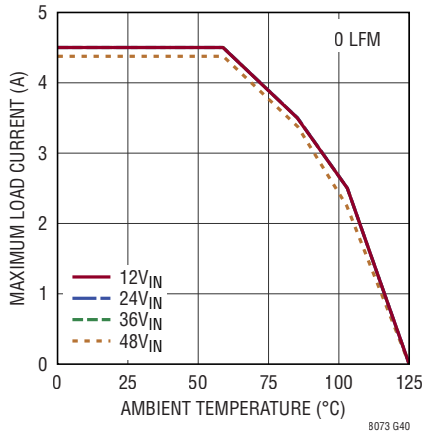
Derating, V_{OUT} = 1V , BIAS = 5V, DC2389A Demo Board
