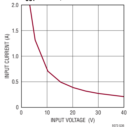
Input Current vs V_{IN} V_{OUT} Shorted, DC2389A Eval Board
