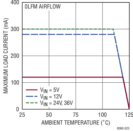
Derating, 1.2 V_{OUT2}
