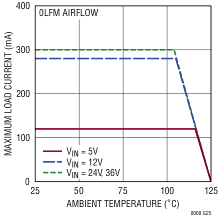
Derating, 1.8 V_{OUT2}
