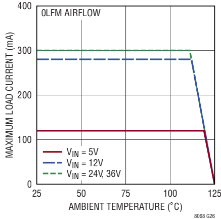
Derating, 2.5 V_{OUT2}
