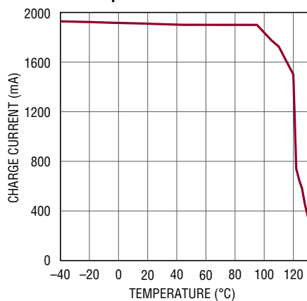
Maximum Charge Current vs Temperature
