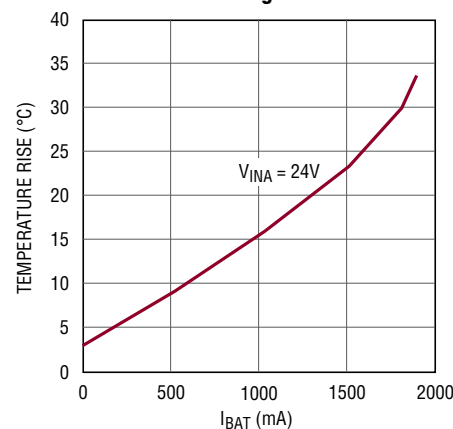
Temperature Rise vs I_{\text{BAT}} , 14.4V Float Voltage
