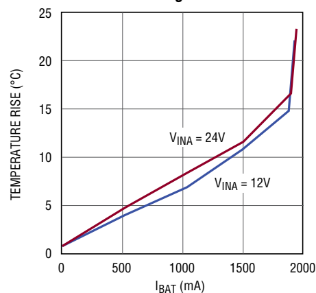
Temperature Rise vs I_{\text{BAT}} , 4.2V Float Voltage
