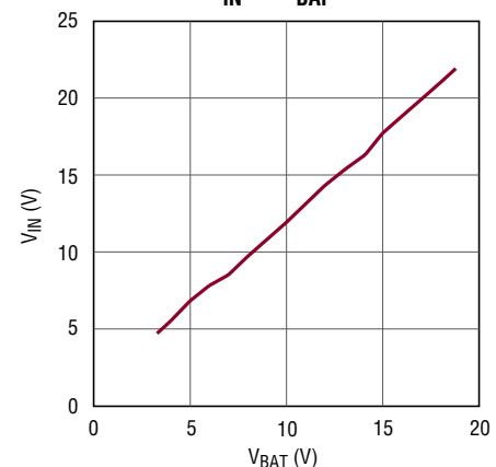
Minimum V_{\text{IN}} vs V_{\text{BAT}} 1.7A Load
