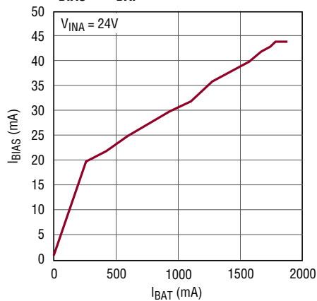
I_{\text{BIAS}} vs I_{\text{BAT}} , 18.8V Float
