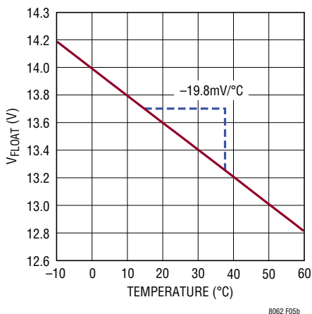
Figure 5. Lead-Acid 6-Cell Float Charge Voltage vs Temperature with a -19.8mV/°C Temperature Coefficient Using LM234 with the Feedback Network
