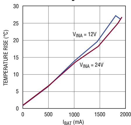
Temperature Rise vs I_{\text{BAT}} , 8.4V Float Voltage
