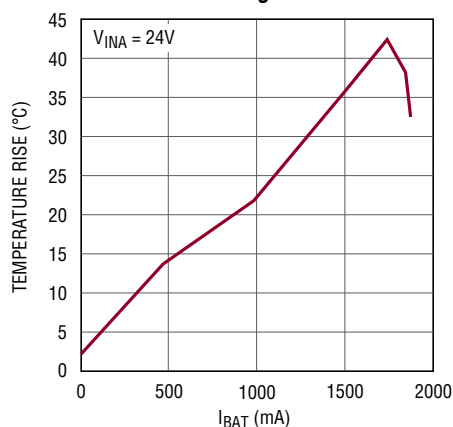
Temperature Rise vs I_{\text{BAT}} , 18.8V Float Voltage
