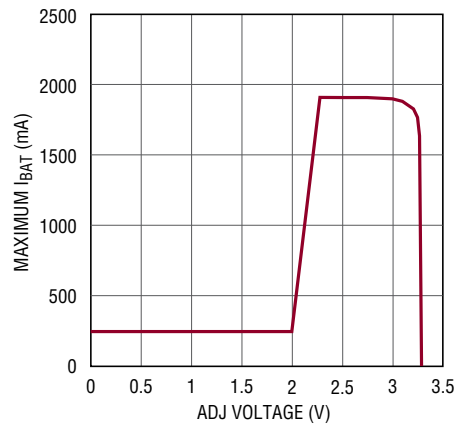
Maximum I_{\text{BAT}} vs ADJ
