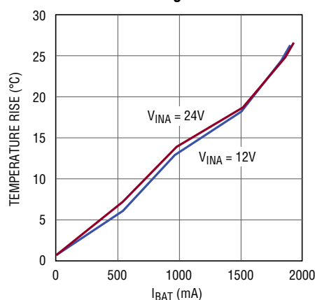
Temperature Rise vs I_{\text{BAT}} , 7.2V Float Voltage
