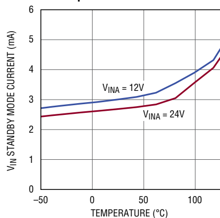
V_{\text{IN}} Standby Mode Current vs Temperature
