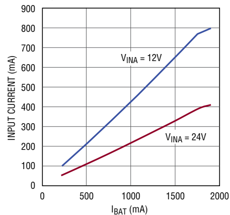
Input Current vs I_{\text{BAT}} , 4.2V Float
