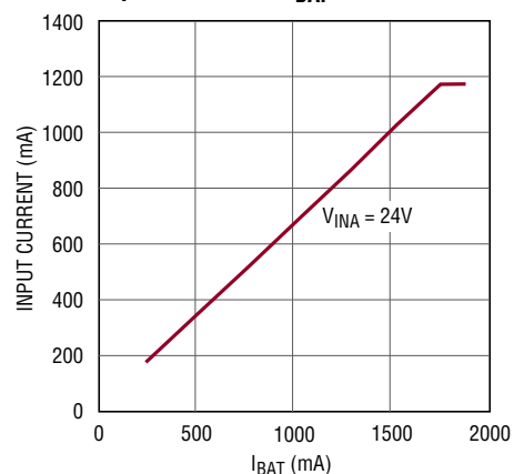
Input Current vs I_{\text{BAT}} , 14.4V Float
