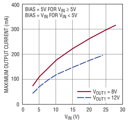
Maximum Output Current vs V_{IN}
