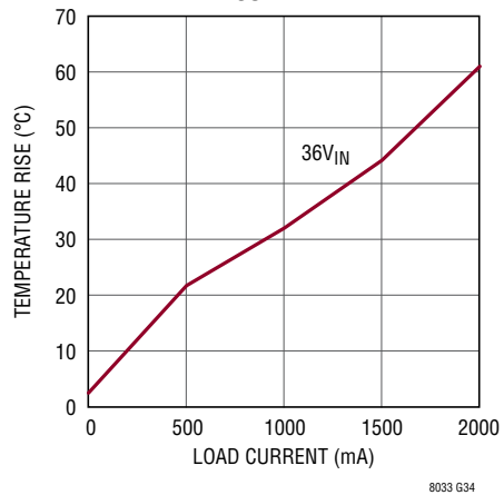
Temperature Rise vs Load Current, 18\text{V}_{\text{OUT}}
