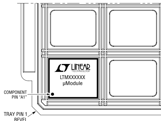
PACKAGE IN TRAY LOADING ORIENTATION
