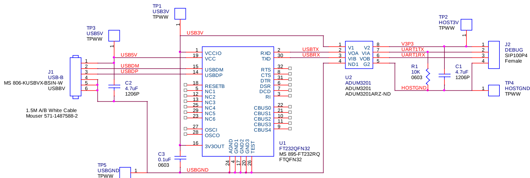
Figure 7: USB Daughter Board Electrical Schematic
