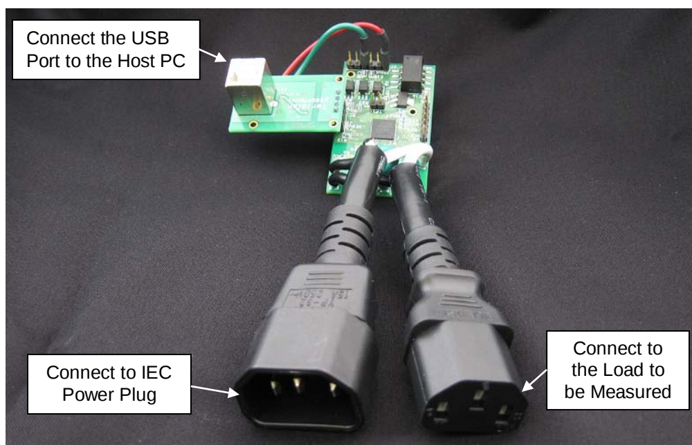
Figure 1: AC-PMON Connections
