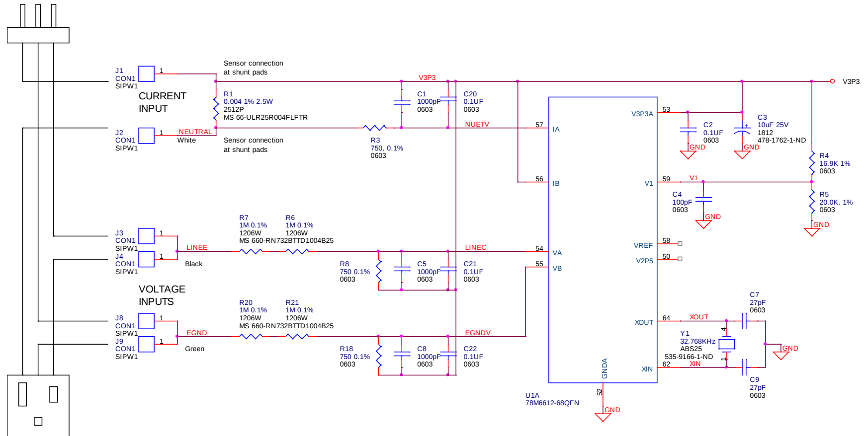
Figure 3: 78M6612 AC-PMON Evaluation Board Electrical Schematic (1 of 2)
