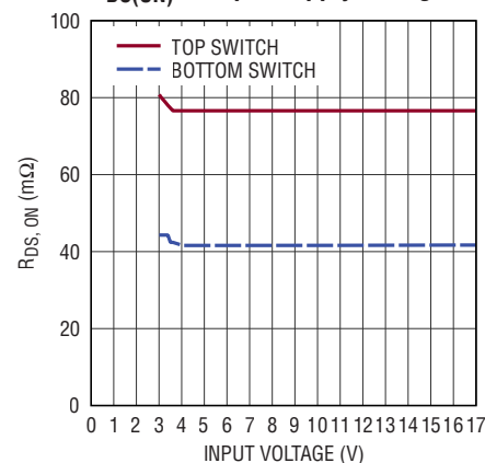
R_{DS(ON)} vs Input Supply Voltage
