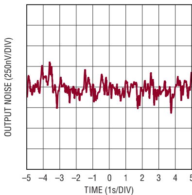
1.25V Low Frequency 0.1Hz to 10Hz Noise
