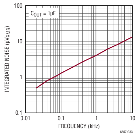
5V Integrated Noise 10Hz to 10kHz
