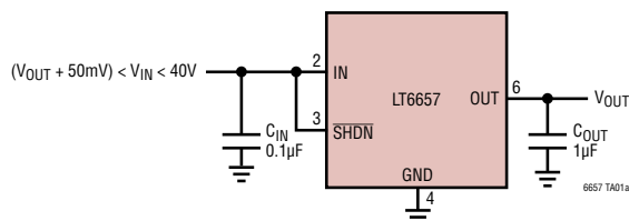
Basic Connection
