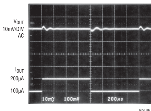
Figure 7. Output Response to Current-Sinking Load Step (100μA to 200μA)
