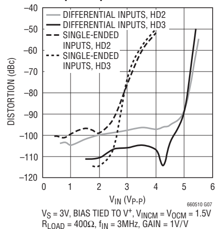
Harmonic Distortion vs Input Amplitude
