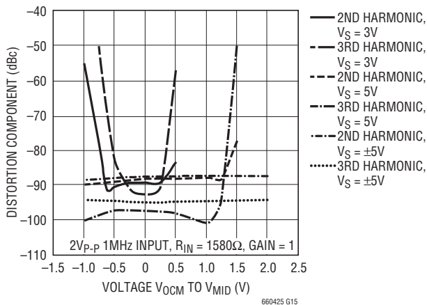
Distortion vs Output Common Mode Level
