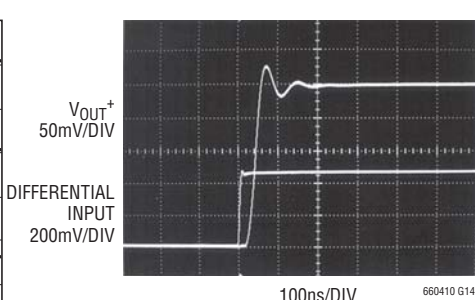
Transient Response, Differential Gain = 1
