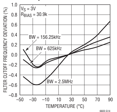
Filter Cutoff Accuracy vs Temperature
