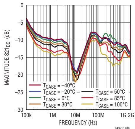
CM to DM Gain (S21 DC ) vs Frequency Over Temperature
