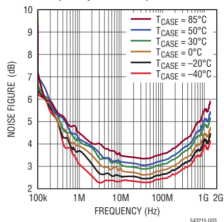
Differential Noise Figure vs Frequency Over Temperature
