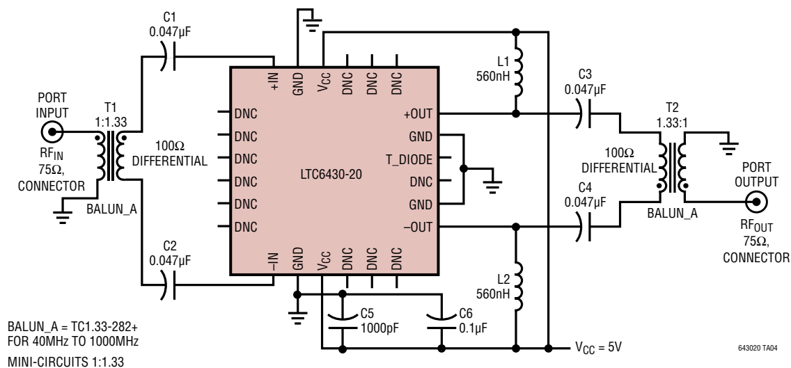
75 \Omega 40MHz to 1000MHz CATV Amplifier
