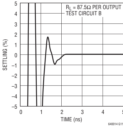
1% Settling Time for 2V Output Step
