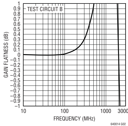
Gain 0.1dB Flatness
