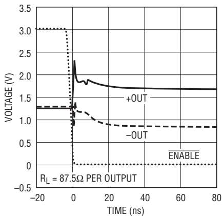
Turn-On Time
