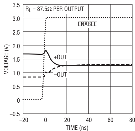
Turn-Off Time
