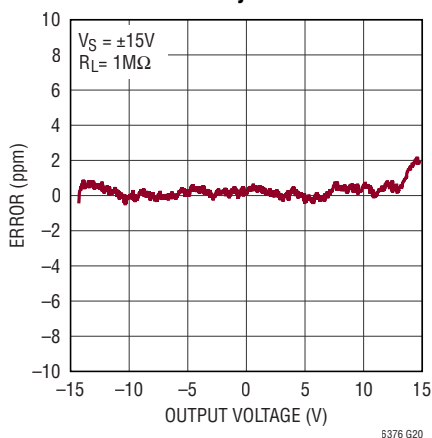
Gain Nonlinearity
