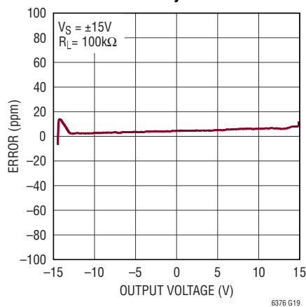
Gain Nonlinearity
