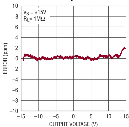
Gain Nonlinearity
