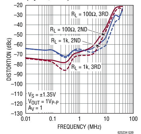
Distortion vs Frequency ( A_V = 1, 2.7V )
