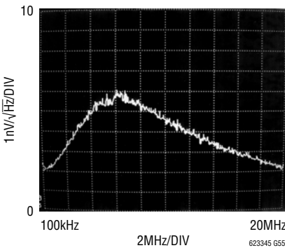
Input Referred High Frequency Noise Spectrum
