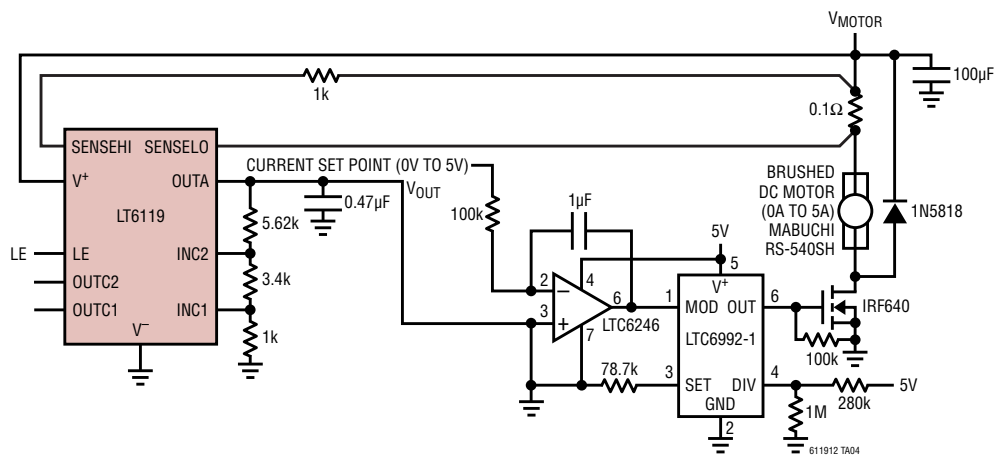
Simplified DC Motor Torque Control
