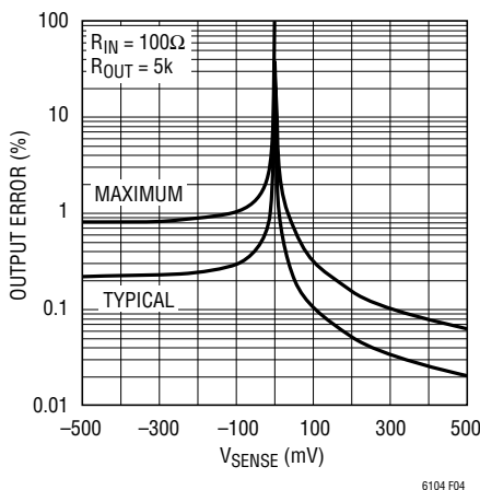
Figure 4. Output Error vs Input Voltage
