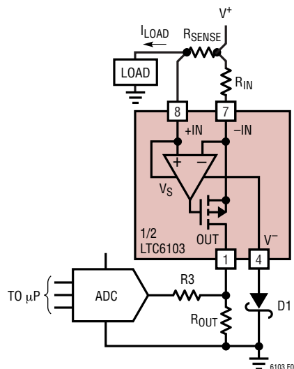
Figure 6. Additional Resistor, R3, Protects Output During Supply Reversal
