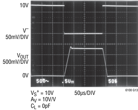
Step Response at V_{SENSE} = 0\text{V} to 130\text{mV}
