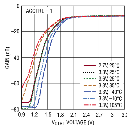
Gain vs V_{CTRL} Voltage
