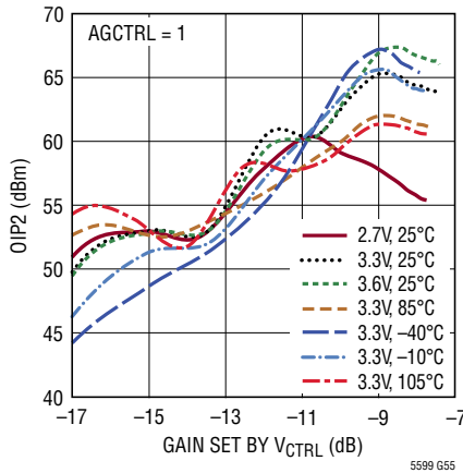
Output IP2 vs V_{CTRL} Gain
