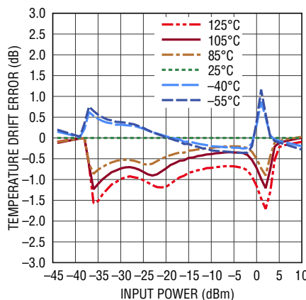
Linearity Error Temperature Variation from 25^\circ C at 12GHz
