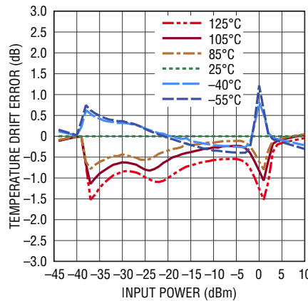
Linearity Error Temperature Variation from 25^\circ C at 5.8GHz
