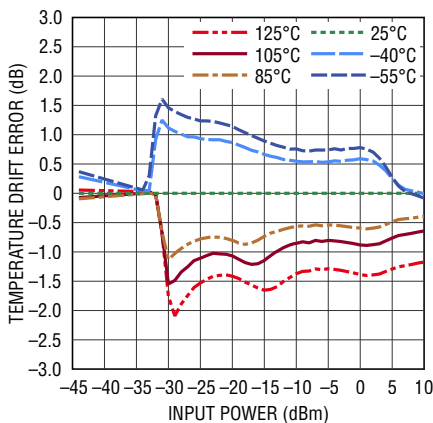
Linearity Error Temperature Variation from 25°C at 40GHz
