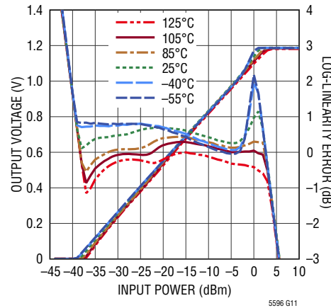
Output Voltage, Linearity Error vs RF Input Power at 24GHz
