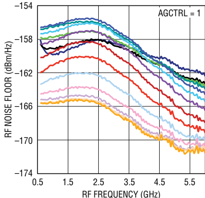
Noise Floor vs RF Frequency and V_{CTRL}
