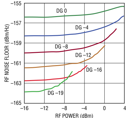
Noise Floor vs RF Power
