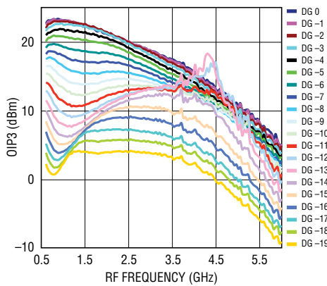
Output IP3 vs RF Frequency and Digital Gain Setting
