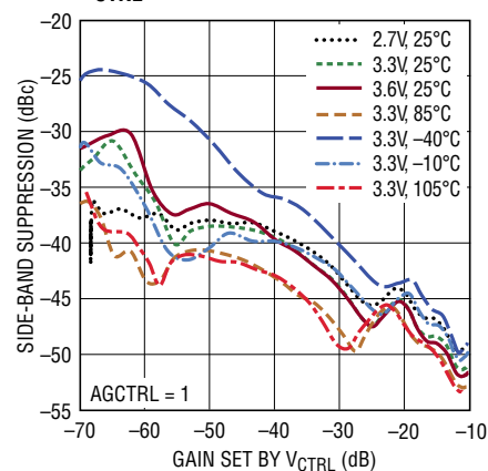
Side-Band Suppression vs V_{CTRL} Gain
