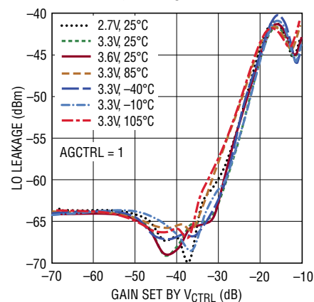
LO Leakage vs V_{CTRL} Gain
