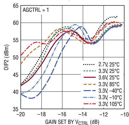
Output IP2 vs V_{CTRL} Gain
