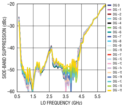
Side-Band Suppression vs LO Frequency and Digital Gain Setting
