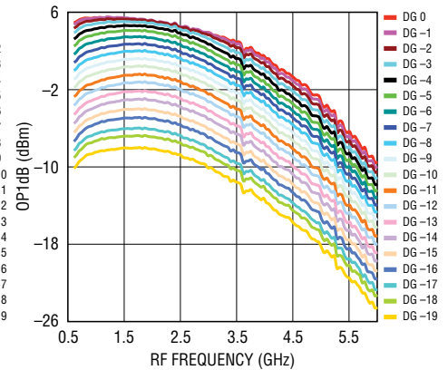
Output 1dB Compression Point vs RF Frequency and Digital Gain Setting at 3.3V Supply, -40^\circ C
