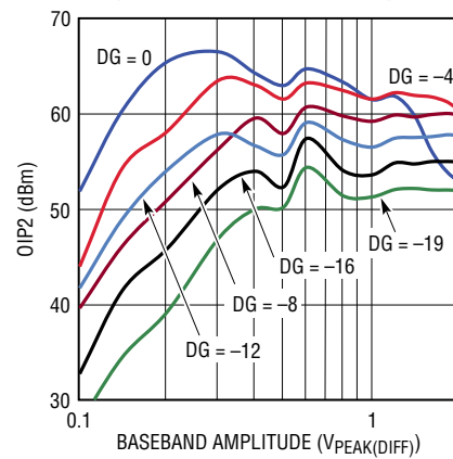
Output IP2 vs Baseband Amplitude
