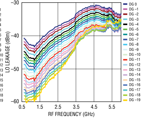
LO Leakage vs RF Frequency and Digital Gain Setting
