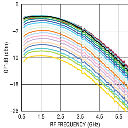
Output 1dB Compression Point vs RF Frequency and Digital Gain Setting at 2.7V Supply, -40^\circ C
