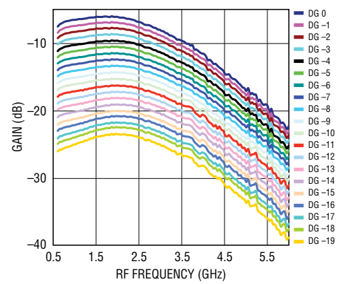
Gain vs RF Frequency and Digital Gain Setting
