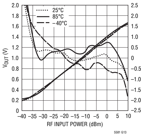
Output Voltage and Linearity Error at 2600MHz
