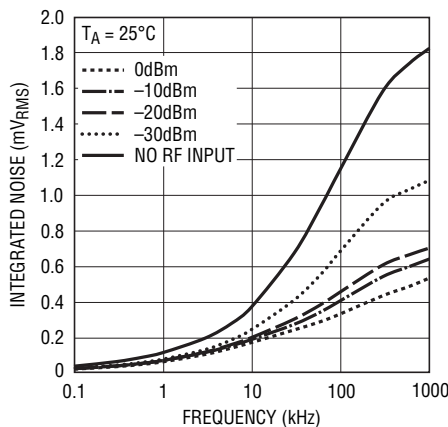
Figure 13. Integrated Output Voltage Noise
