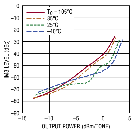
2-Tone IM3 Level vs Output Power Level
